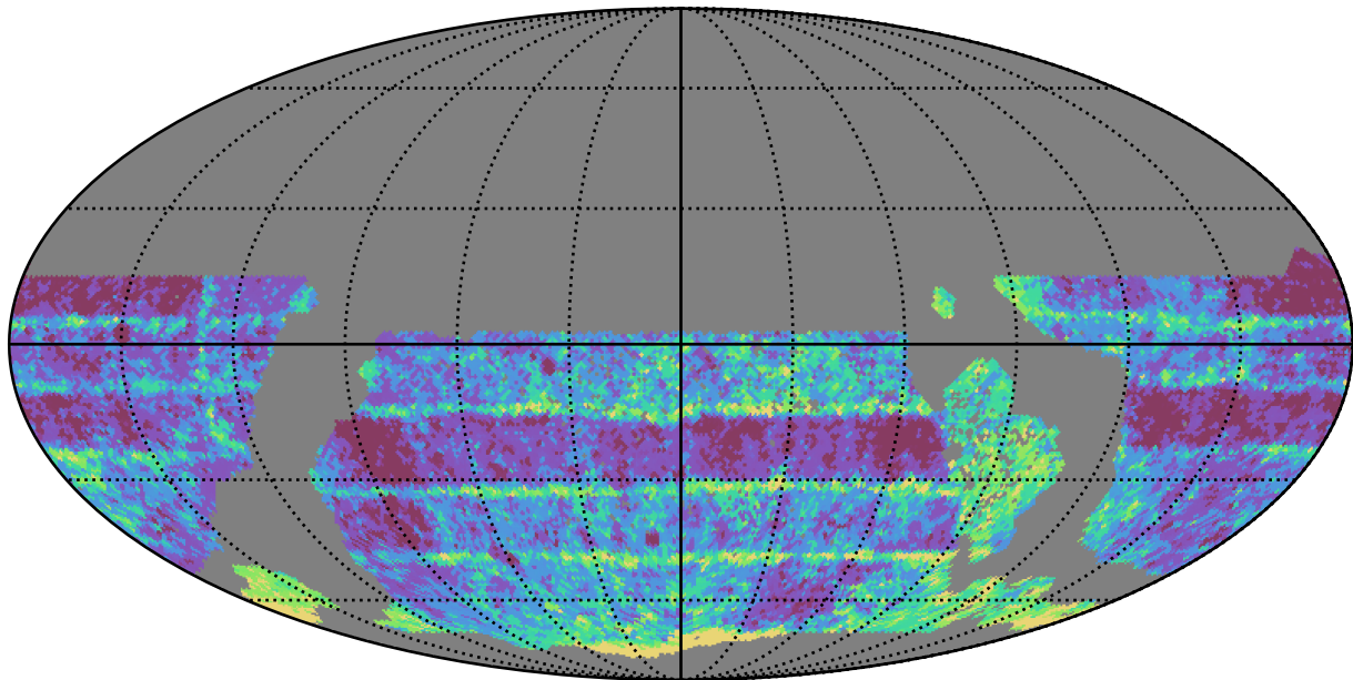
ddf_acor_sf15_lsf30_lsr20_v3.4_10yrs WFD r band: Median Inter-Night Gap
