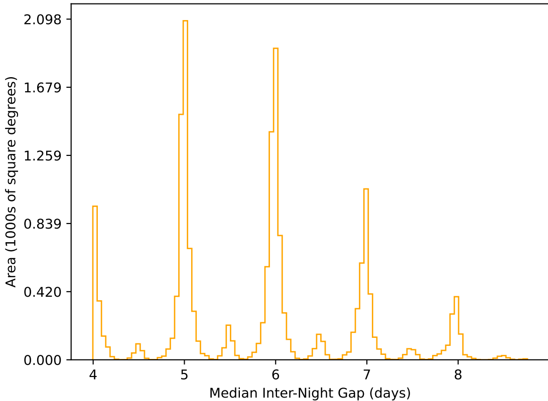
ddf_acor_sf15_lsf30_lsr20_v3.4_10yrs WFD r band: Median Inter-Night Gap
