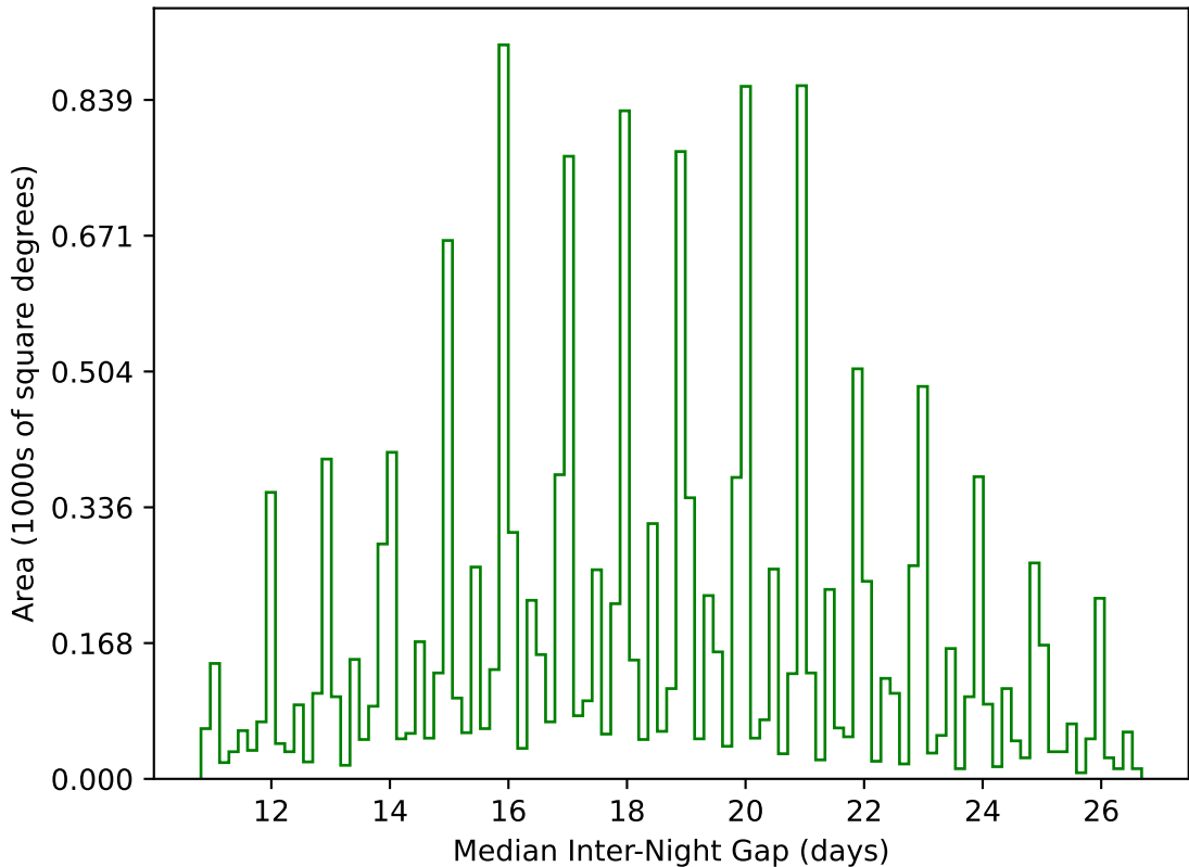
ddf_acor_sf15_lsf30_lsr20_v3.4_10yrs WFD g band: Median Inter-Night Gap
