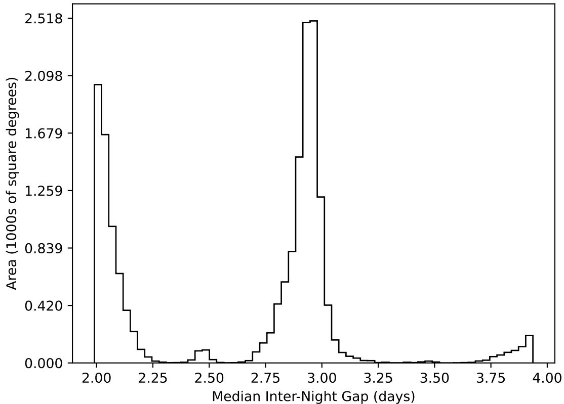
ddf_acor_sf15_lsf30_lsr20_v3.4_10yrs WFD all bands: Median Inter-Night Gap
