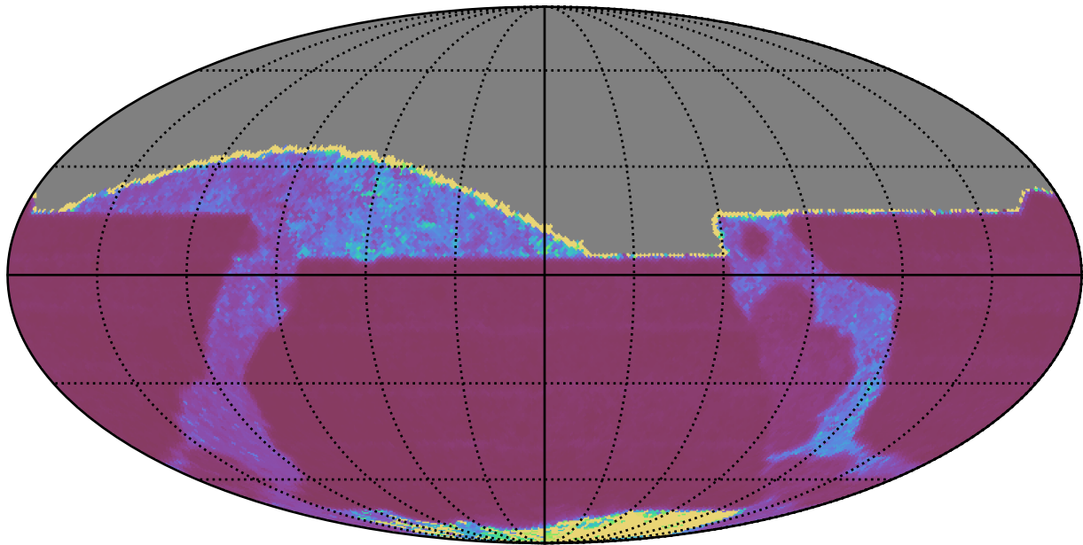
ddf_acor_sf15_lsf30_lsr20_v3.4_10yrs All sky z band: Median Inter-Night Gap
