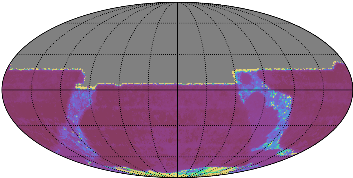
ddf_acor_sf15_lsf30_lsr20_v3.4_10yrs All sky y band: Median Inter-Night Gap
