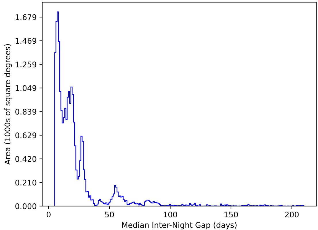
ddf_acor_sf15_lsf30_lsr20_v3.4_10yrs All sky y band: Median Inter-Night Gap
