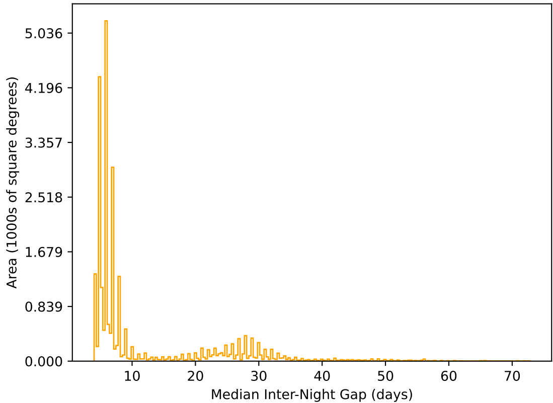
ddf_acor_sf15_lsf30_lsr20_v3.4_10yrs All sky r band: Median Inter-Night Gap
