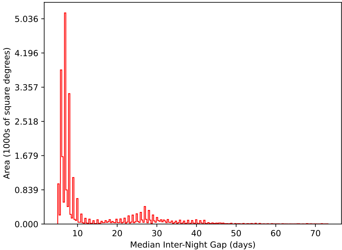
ddf_acor_sf15_lsf30_lsr20_v3.4_10yrs All sky i band: Median Inter-Night Gap
