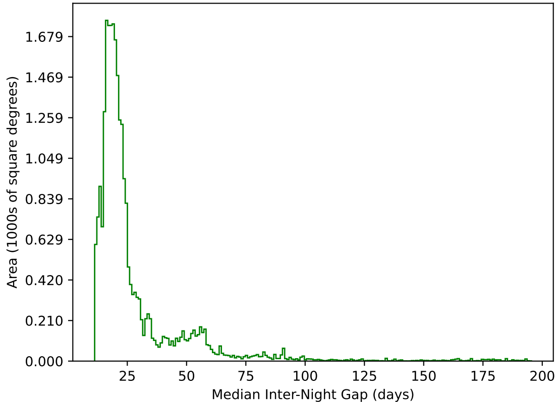
ddf_acor_sf15_lsf30_lsr20_v3.4_10yrs All sky g band: Median Inter-Night Gap
