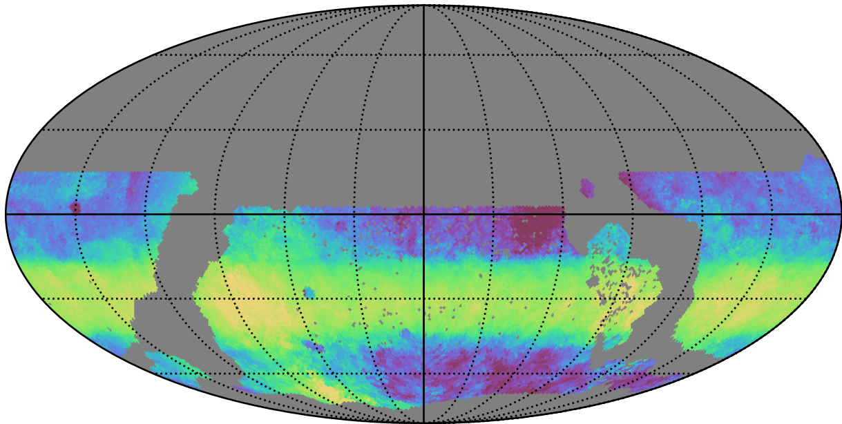
ddf_acor_sf15_lsf30_lsr20_v3.4_10yrs WFD y band: Median HA
