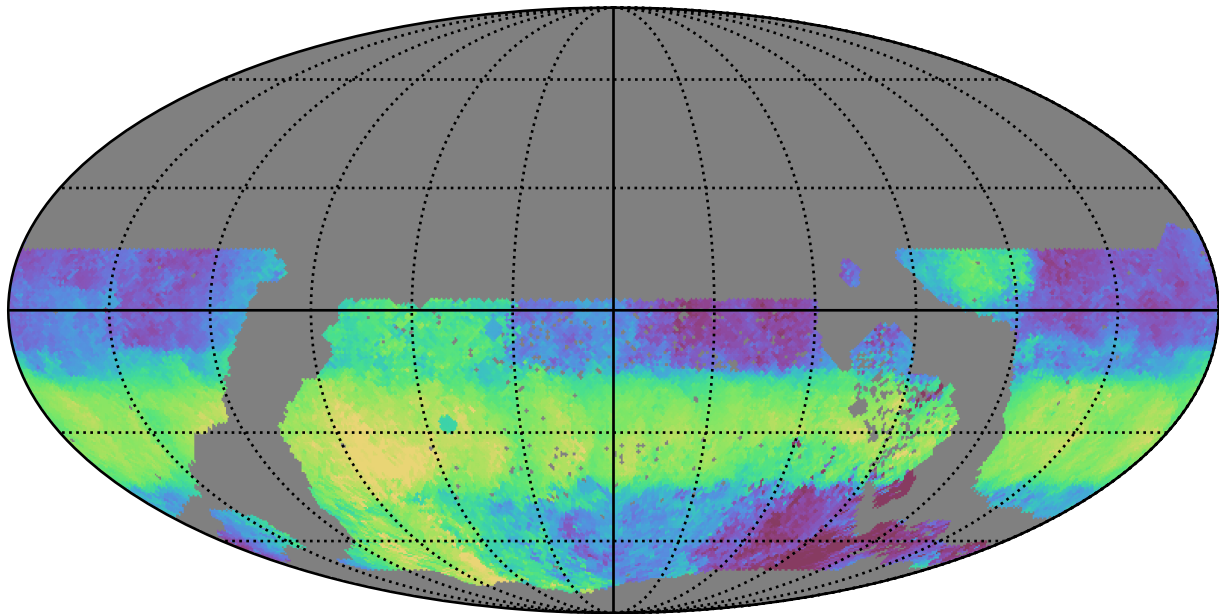
ddf_acor_sf15_lsf30_lsr20_v3.4_10yrs WFD u band: Median HA
