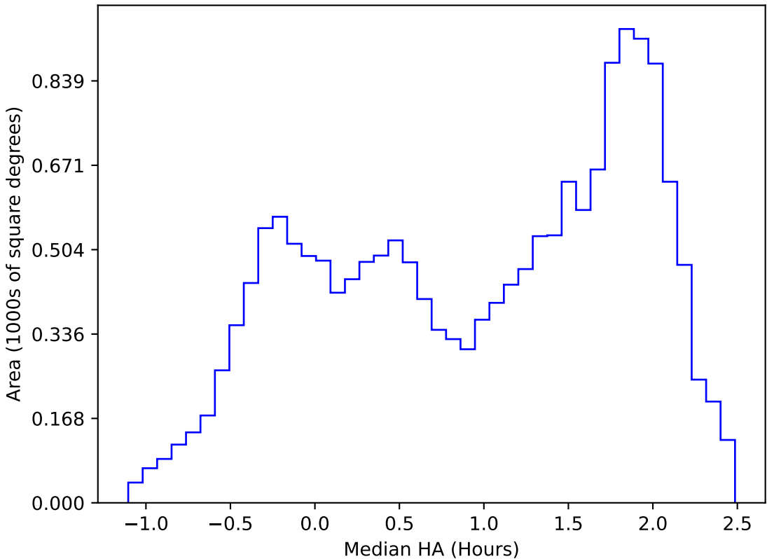
ddf_acor_sf15_lsf30_lsr20_v3.4_10yrs WFD u band: Median HA
