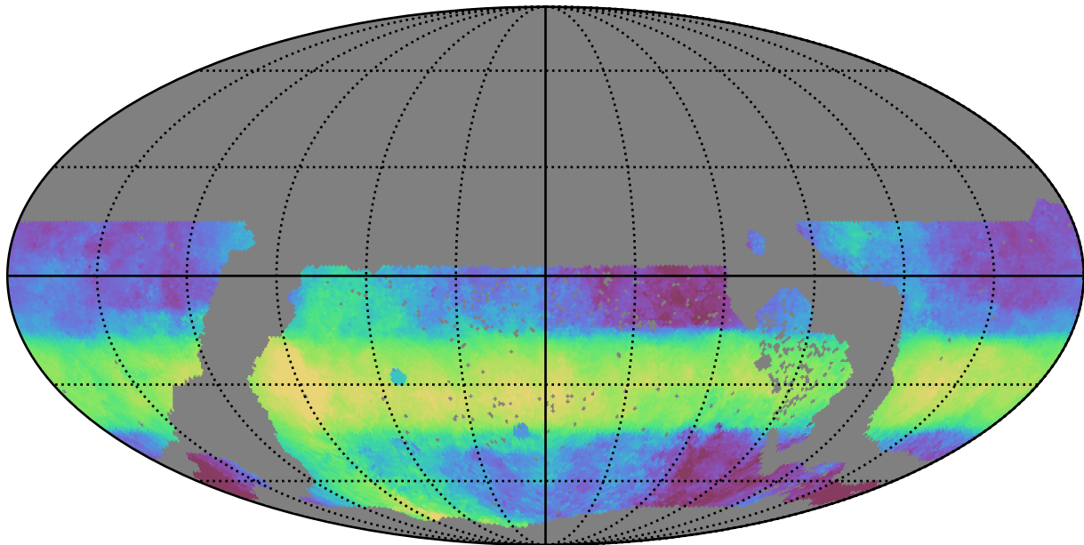
ddf_acor_sf15_lsf30_lsr20_v3.4_10yrs WFD r band: Median HA
