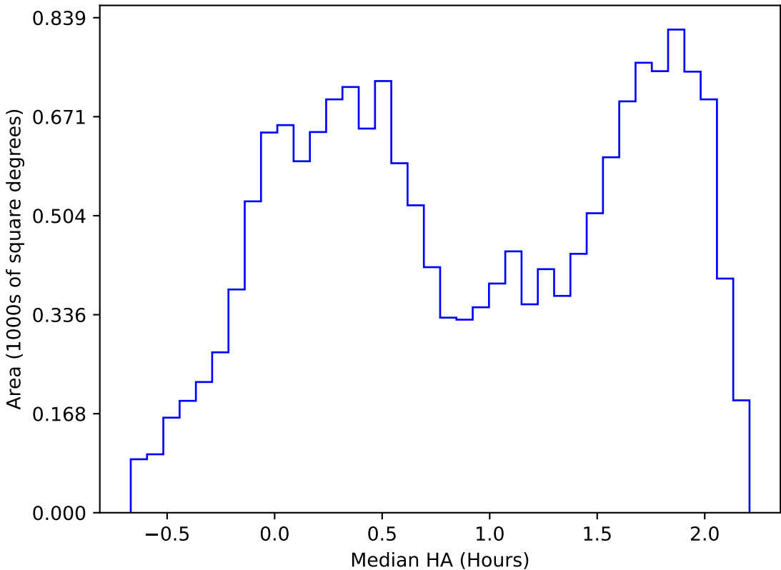
ddf_acor_sf15_lsf30_lsr20_v3.4_10yrs WFD r band: Median HA
