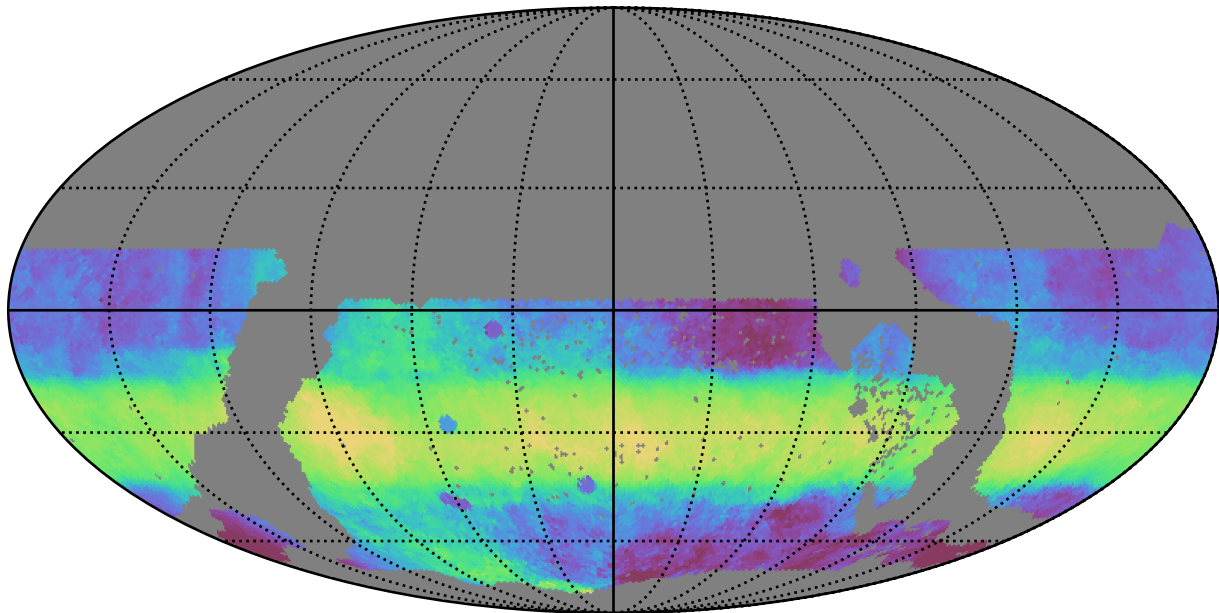
ddf_acor_sf15_lsf30_lsr20_v3.4_10yrs WFD i band: Median HA
