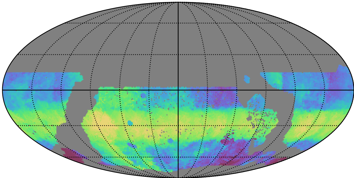
ddf_acor_sf15_lsf30_lsr20_v3.4_10yrs WFD g band: Median HA
