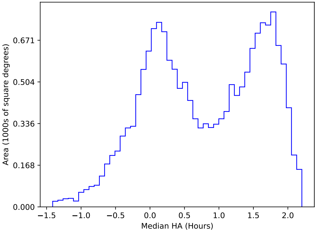
ddf_acor_sf15_lsf30_lsr20_v3.4_10yrs WFD g band: Median HA
