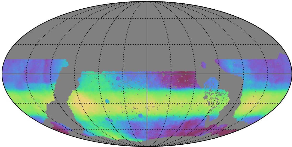
ddf_acor_sf15_lsf30_lsr20_v3.4_10yrs WFD all bands: Median HA
