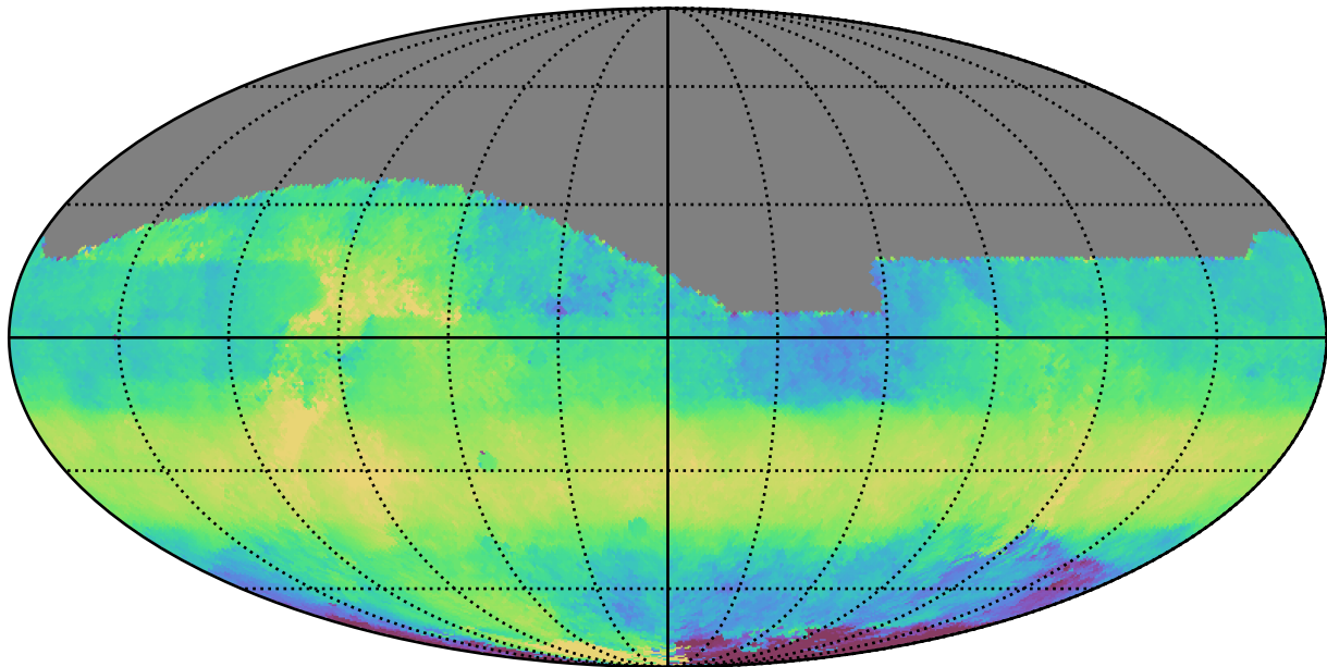
ddf_acor_sf15_lsf30_lsr20_v3.4_10yrs All sky z band: Median HA
