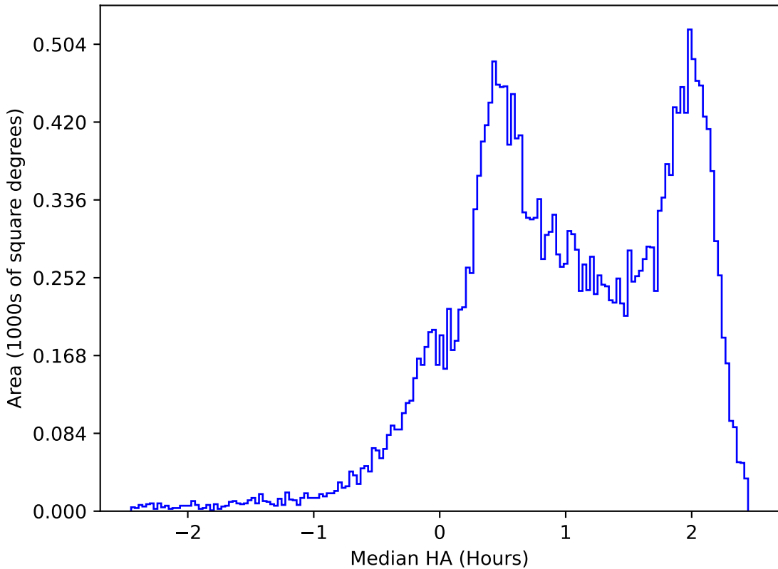
ddf_acor_sf15_ls30_lsr20_v3.4_10yrs All sky z band: Median HA
