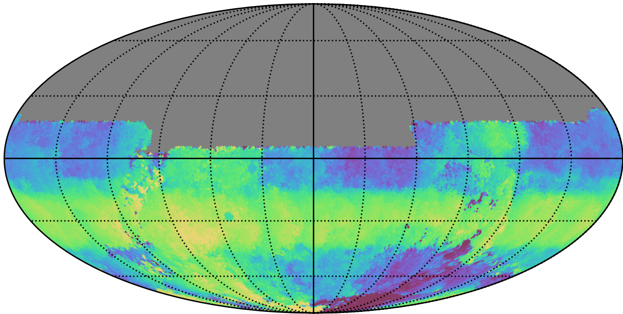
ddf_acor_sf15_lsf30_lsr20_v3.4_10yrs All sky u band: Median HA
