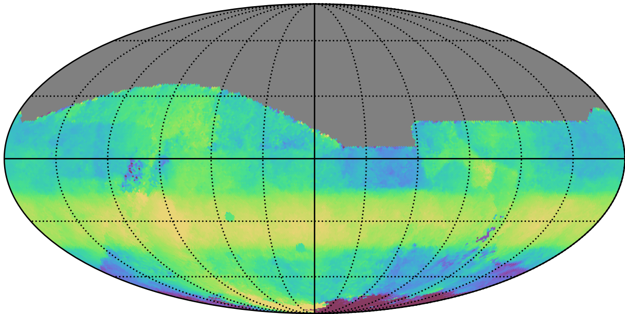
ddf_acor_sf15_lsf30_lsr20_v3.4_10yrs All sky r band: Median HA
