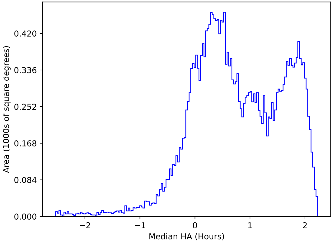
ddf_acor_sf15_lsf30_lsr20_v3.4_10yrs All sky r band: Median HA
