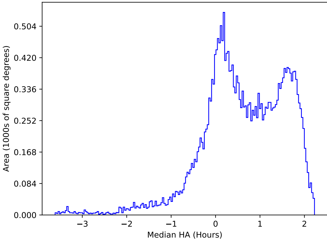
ddf_acor_sf15_ls30_lsr20_v3.4_10yrs All sky g band: Median HA
