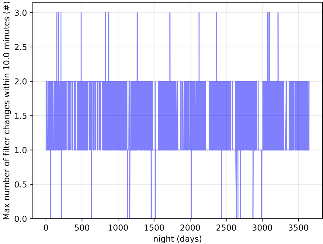
ddf_acor_sf15_Isf30_Isr20_v3.4_10yrs Per Night: Max number of filter changes within 10.0 minutes
