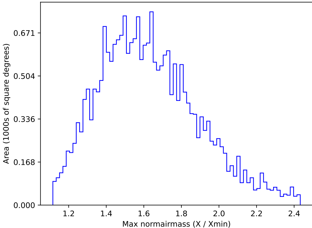
ddf_acor_sf15_lsf30_lsr20_v3.4_10yrs All sky u band: Max normairmass
