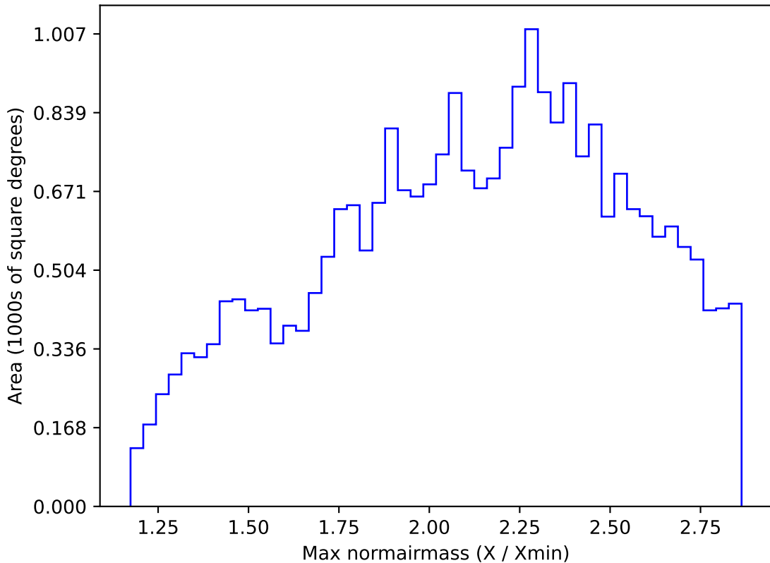
ddf_acor_sf15_lsf30_lsr20_v3.4_10yrs All sky i band: Max normairmass
