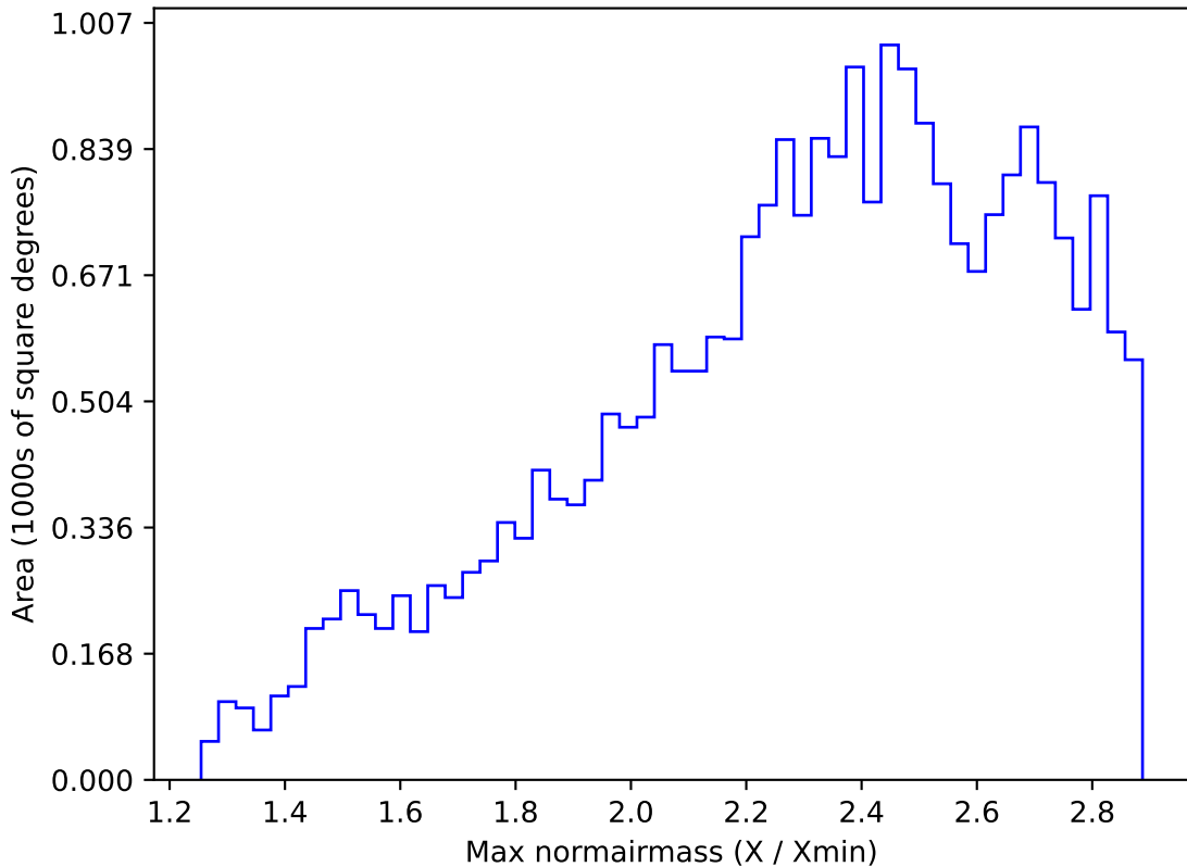
ddf_acor_sf15_lsf30_lsr20_v3.4_10yrs All sky all bands: Max normairmass
