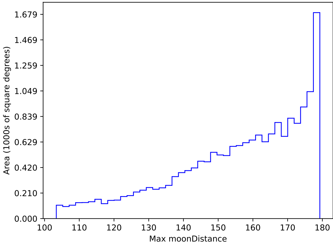
ddf_acor_sf15_lsf30_lsr20_v3.4_10yrs WFD r band: Max moonDistance
