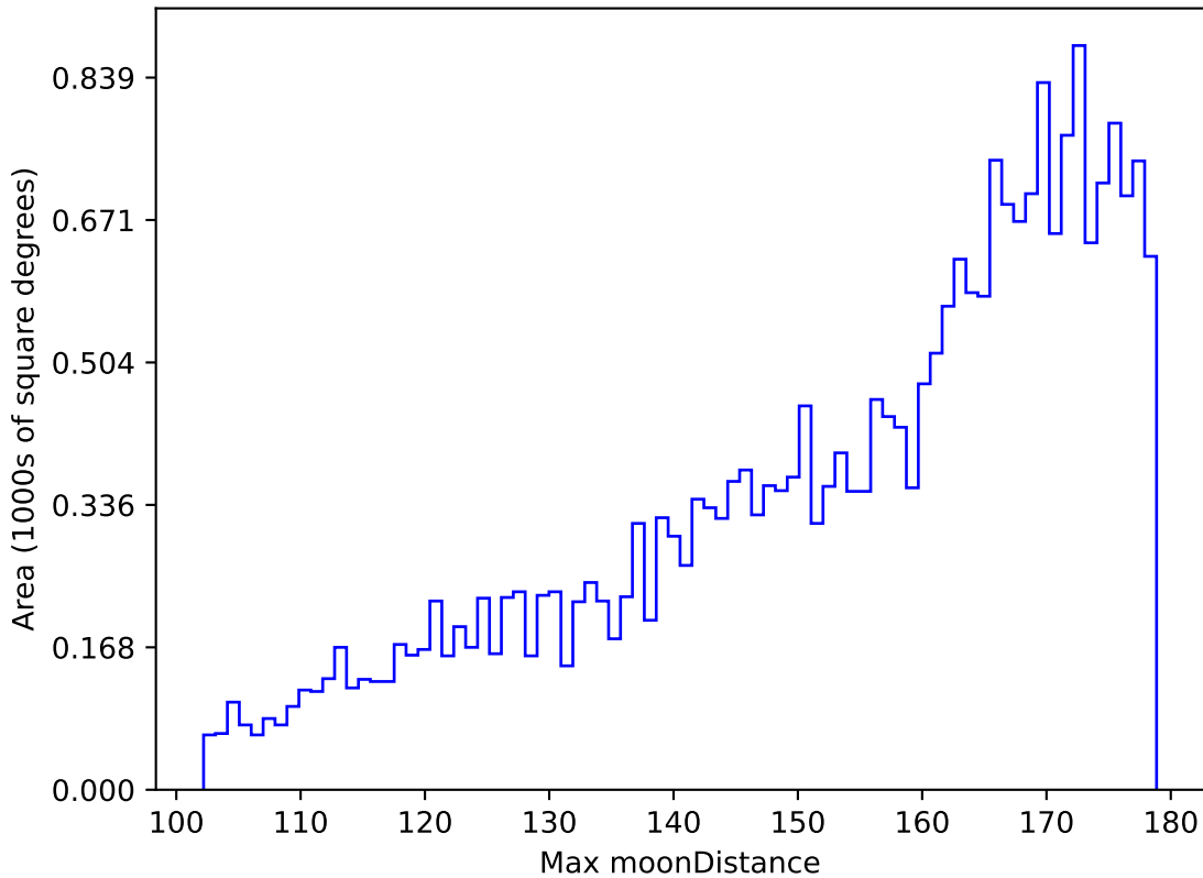
ddf_acor_sf15_lsf30_lsr20_v3.4_10yrs All sky z band: Max moonDistance
