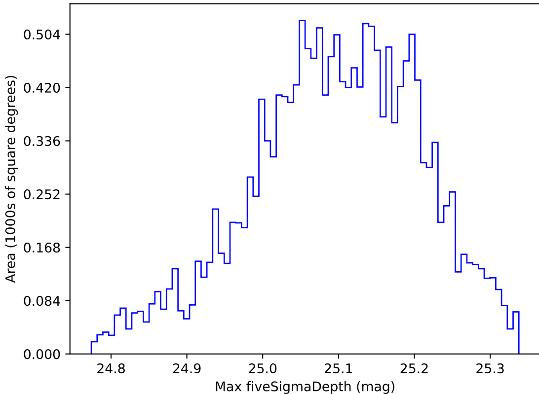
ddf_acor_sf15_lsf30_lsr20_v3.4_10yrs WFD all bands: Max fiveSigmaDepth
