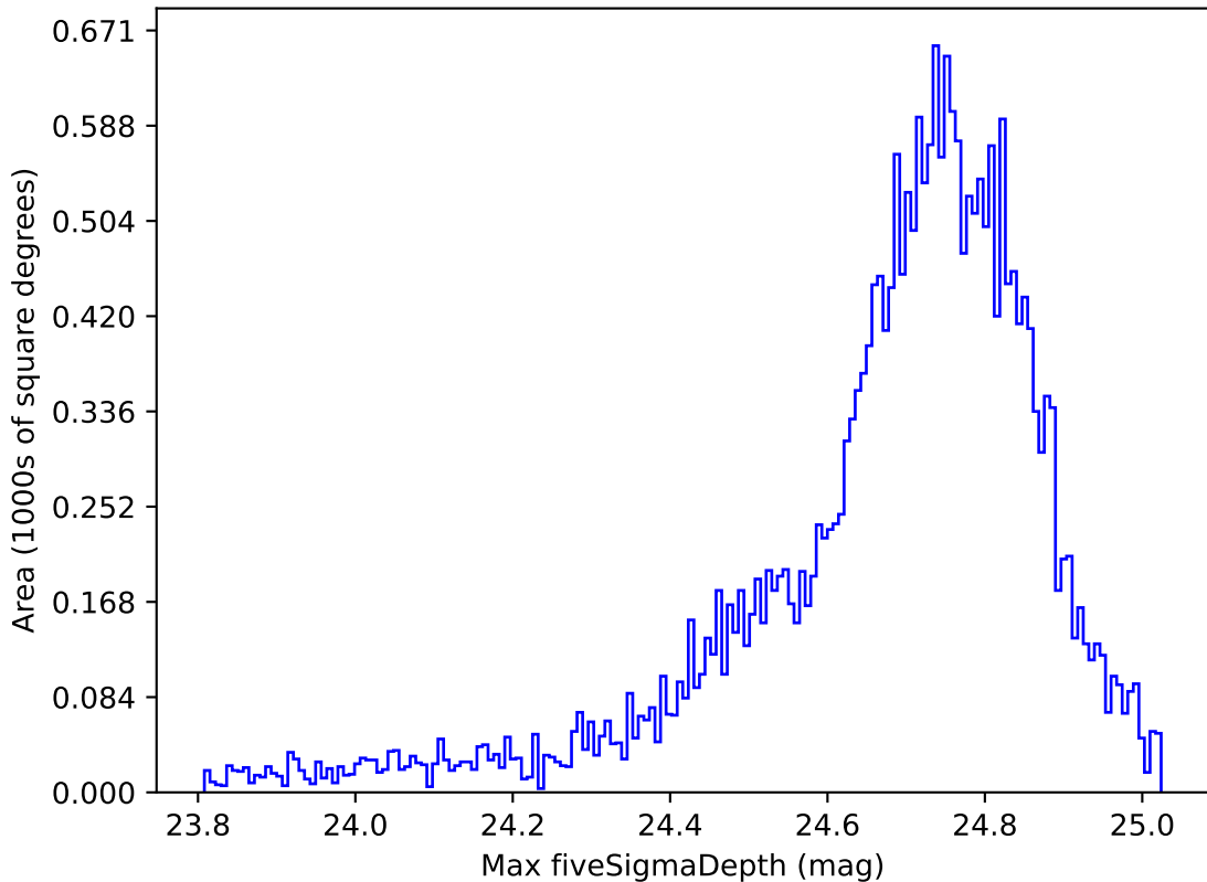
ddf_acor_sf15_lsf30_lsr20_v3.4_10yrs All sky r band: Max fiveSigmaDepth
