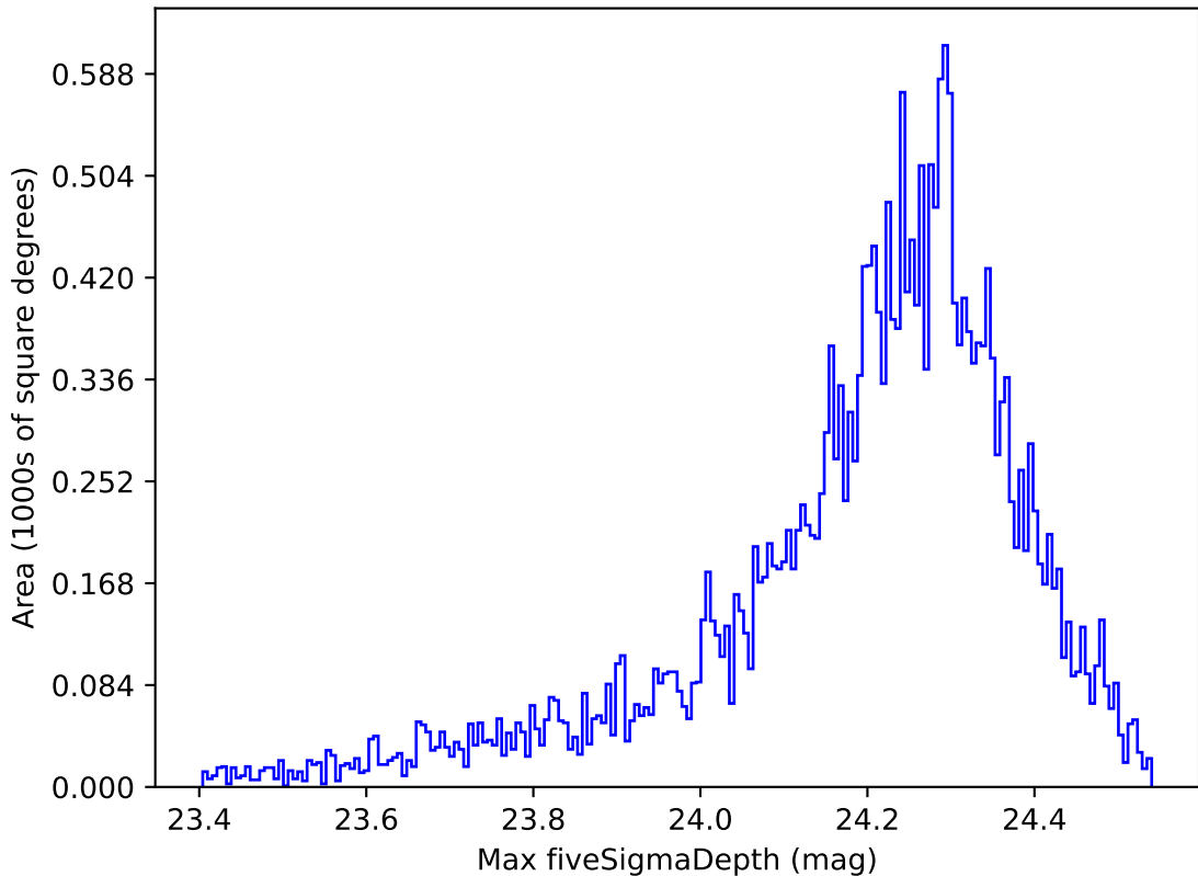
ddf_acor_sf15_lsf30_lsr20_v3.4_10yrs All sky i band: Max fiveSigmaDepth
