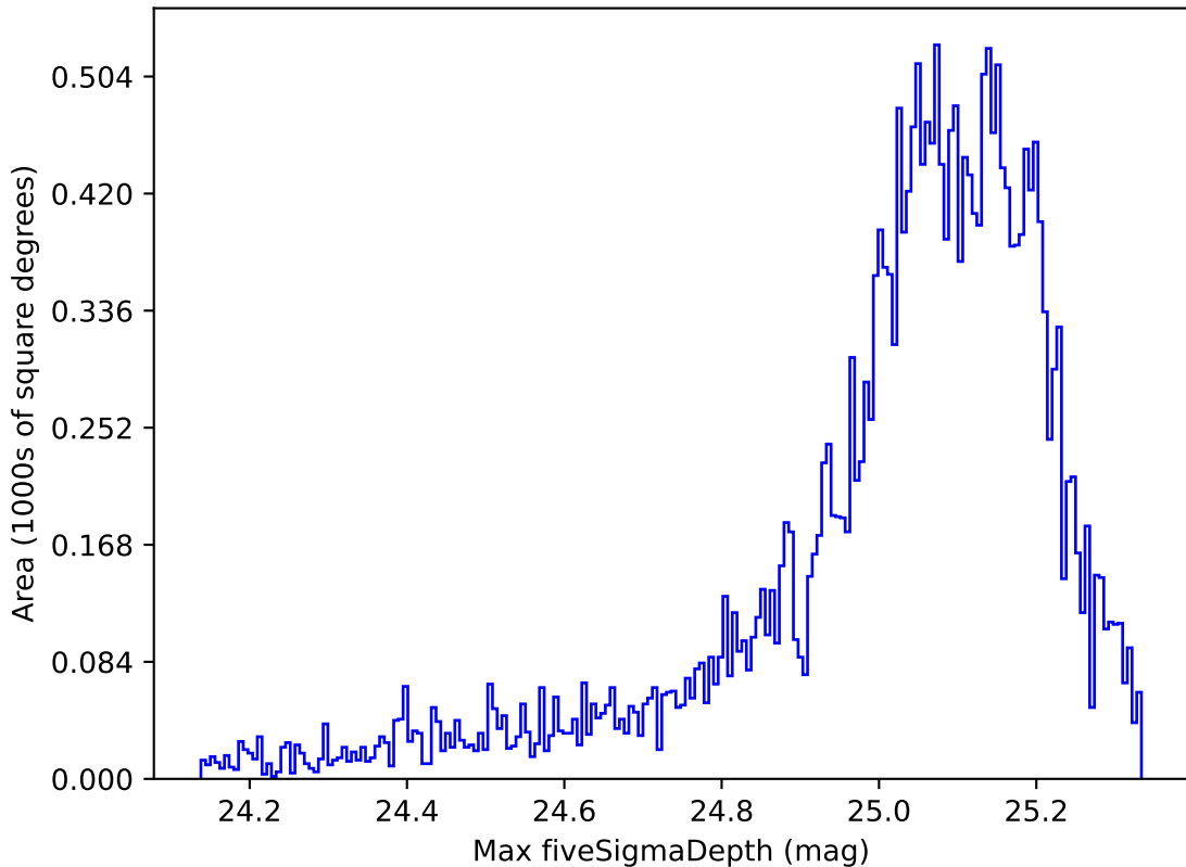
ddf_acor_sf15_ls30_lsr20_v3.4_10yrs All sky g band: Max fiveSigmaDepth
