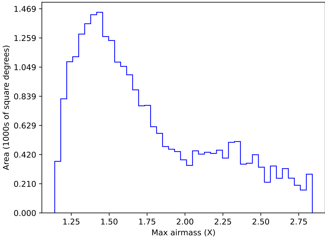
ddf_acor_sf15_lsf30_lsr20_v3.4_10yrs Yr 1 z band: Max airmass
