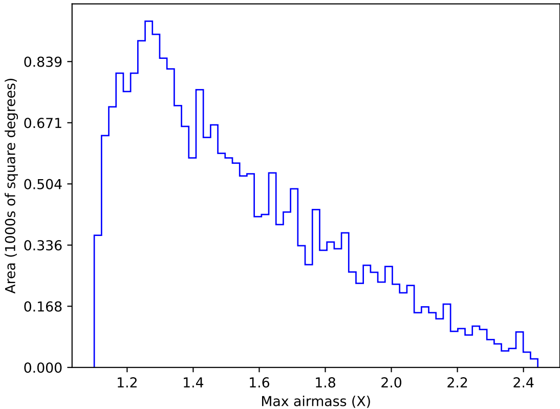
ddf_acor_sf15_lsf30_lsr20_v3.4_10yrs Yr 1 u band: Max airmass
