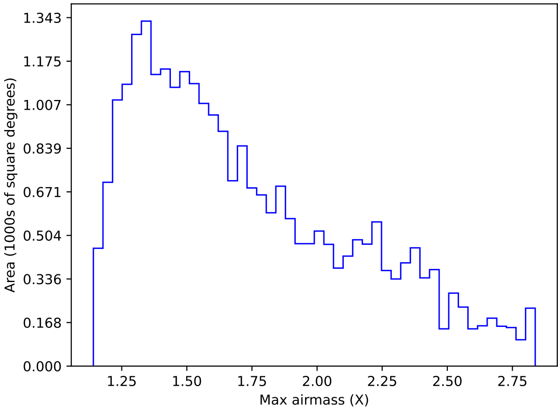
ddf_acor_sf15_lsf30_lsr20_v3.4_10yrs Yr 1 i band: Max airmass
