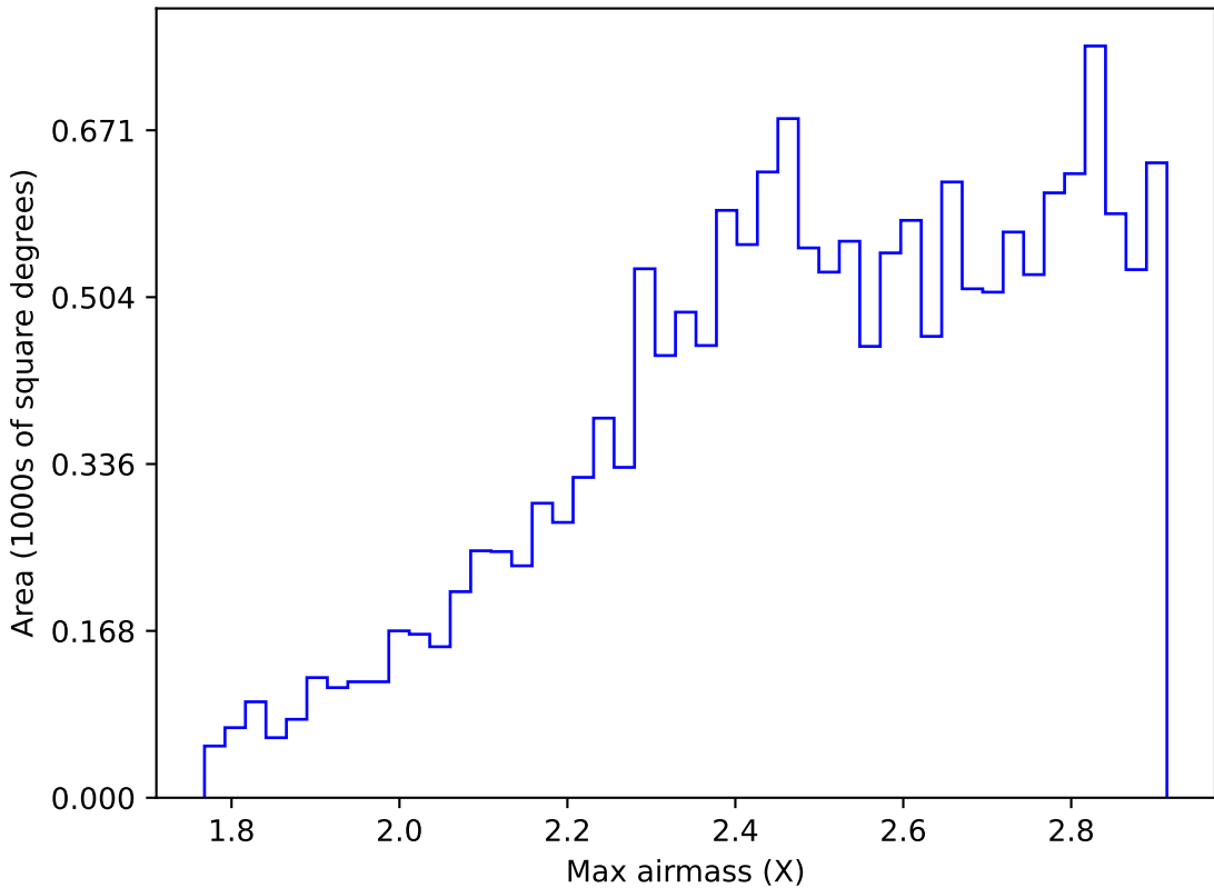
ddf_acor_sf15_ls30_lsr20_v3.4_10yrs WFD z band: Max airmass
