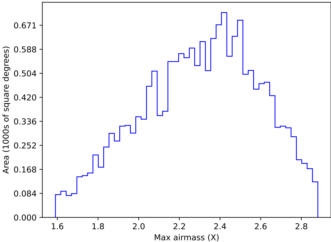
ddf_acor_sf15_ls30_lsr20_v3.4_10yrs WFD y band: Max airmass
