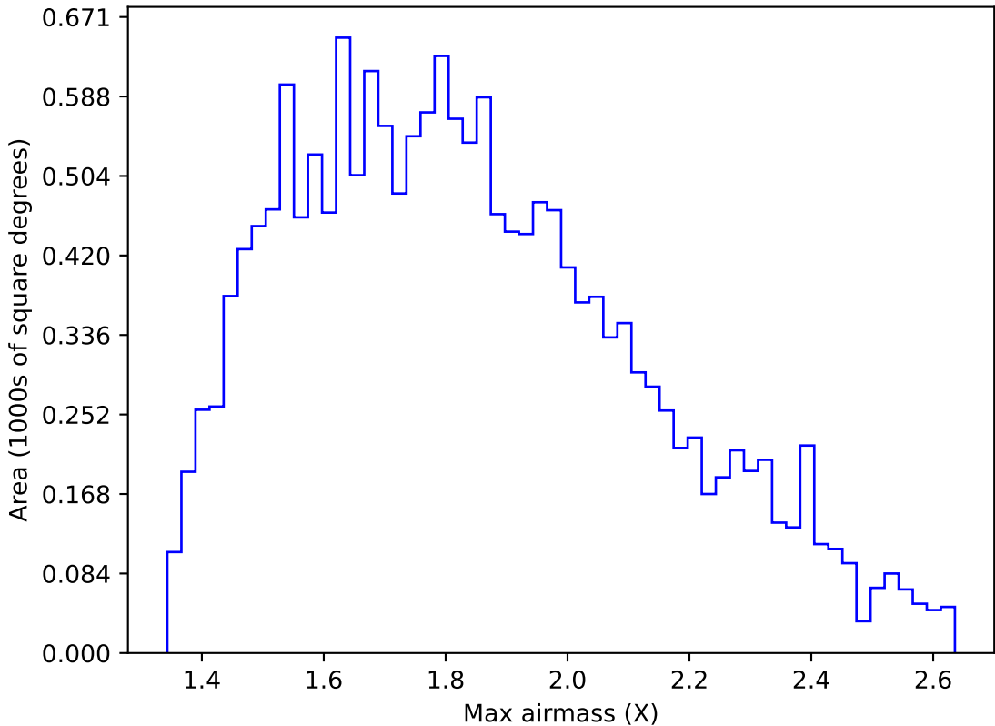
ddf_acor_sf15_lsf30_lsr20_v3.4_10yrs WFD u band: Max airmass
