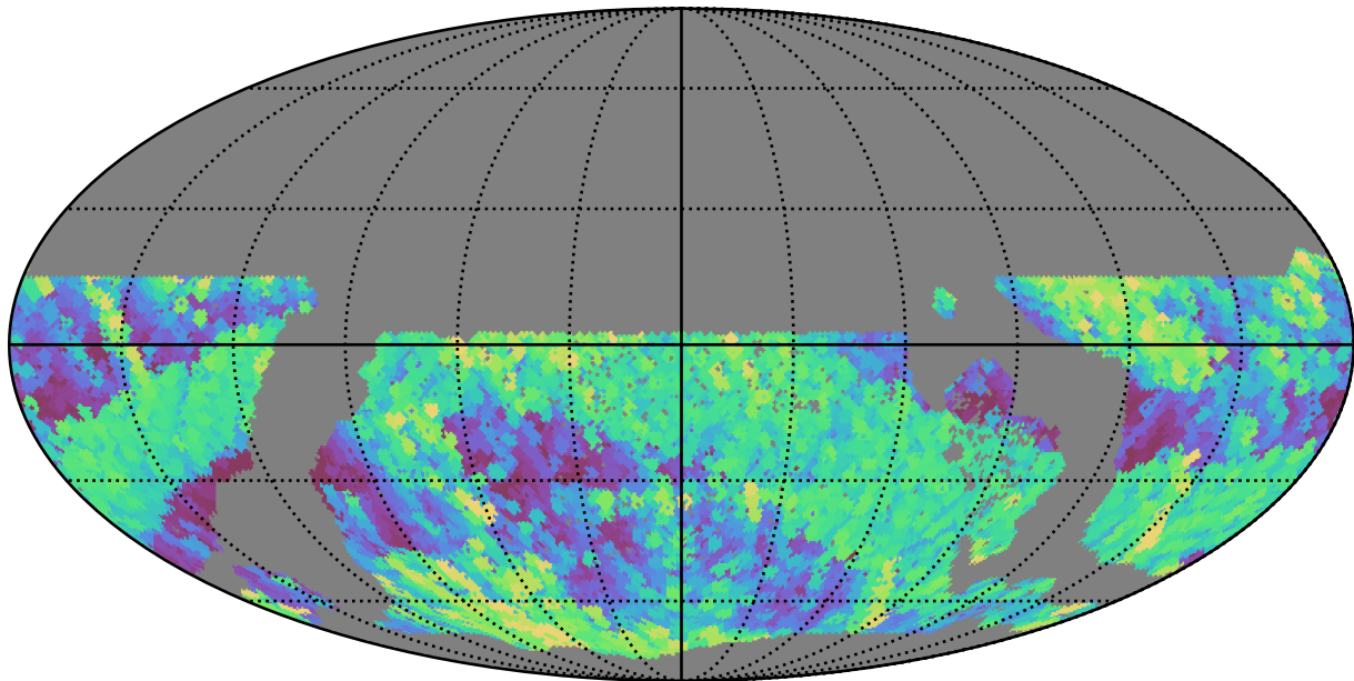
ddf_acor_sf15_lsf30_lsr20_v3.4_10yrs WFD r band: Max airmass
