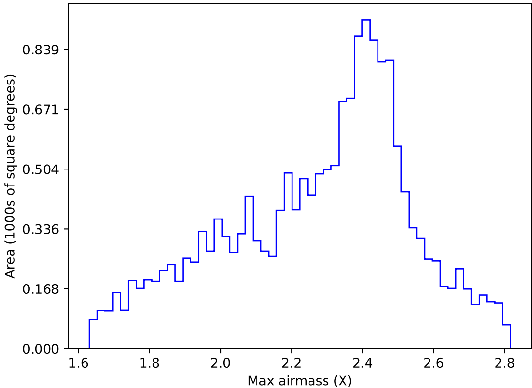
ddf_acor_sf15_lsf30_lsr20_v3.4_10yrs WFD r band: Max airmass
