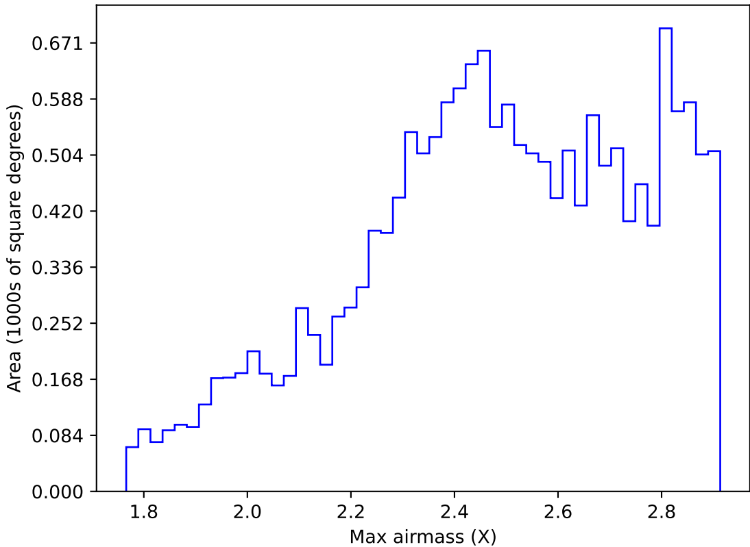
ddf_acor_sf15_lsf30_lsr20_v3.4_10yrs WFD i band: Max airmass
