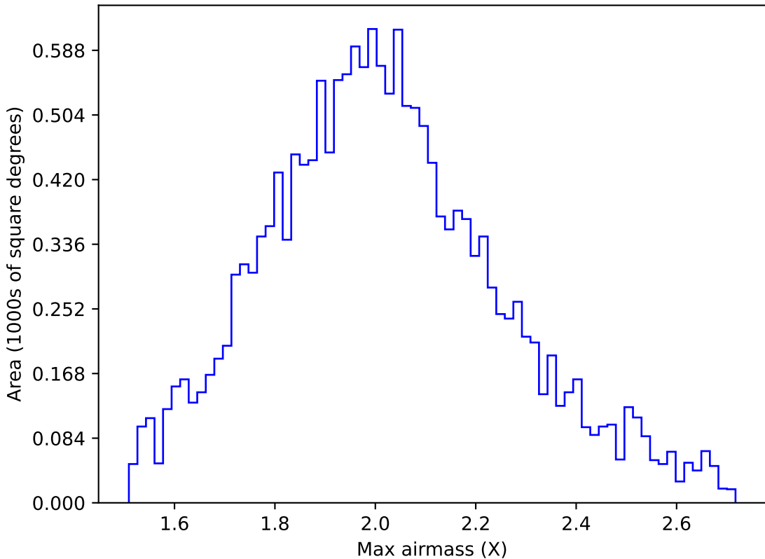
ddf_acor_sf15_lsf30_lsr20_v3.4_10yrs WFD g band: Max airmass
