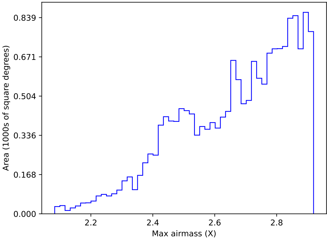
ddf_acor_sf15_lsf30_lsr20_v3.4_10yrs WFD all bands: Max airmass
