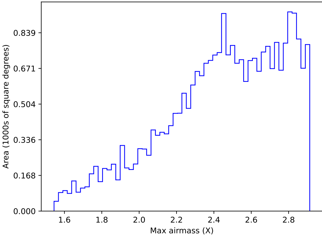
ddf_acor_sf15_lsf30_lsr20_v3.4_10yrs All sky z band: Max airmass
