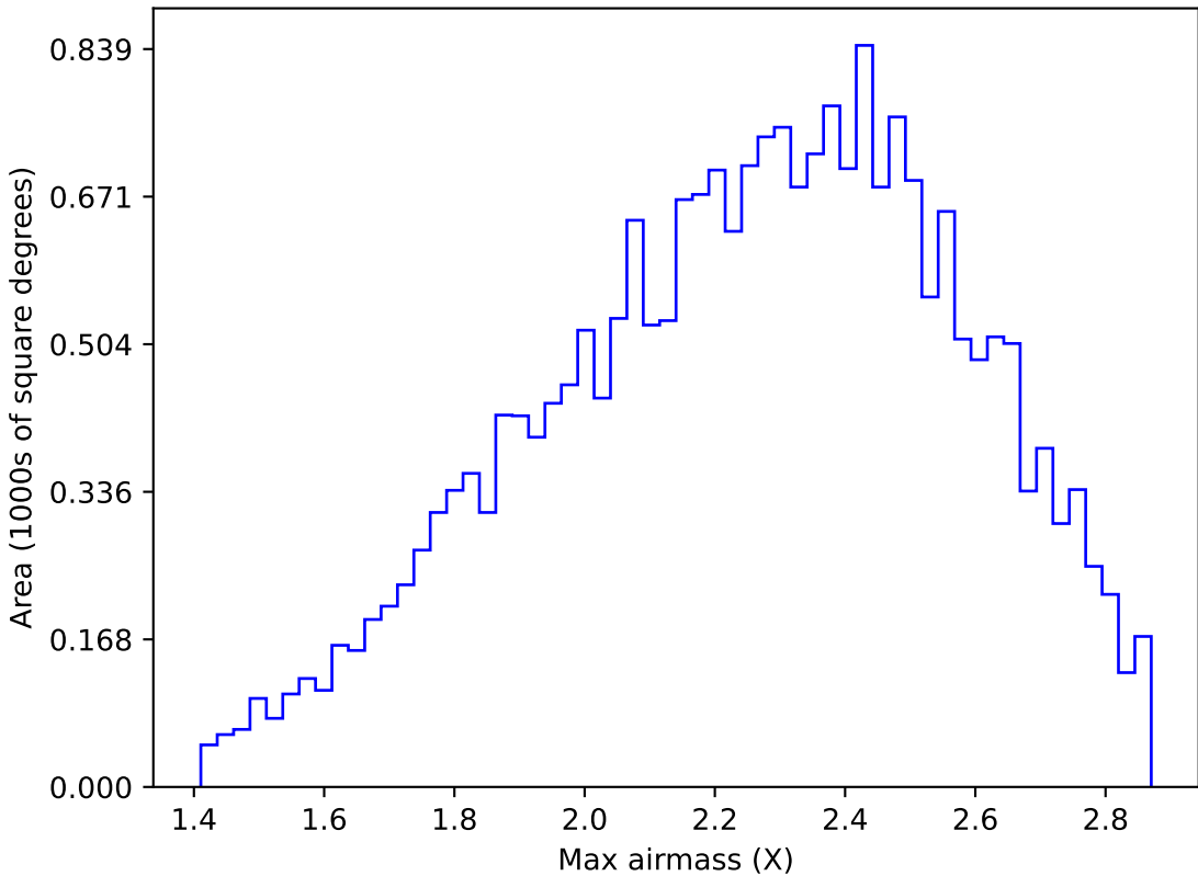
ddf_acor_sf15_lsf30_lsr20_v3.4_10yrs All sky y band: Max airmass
