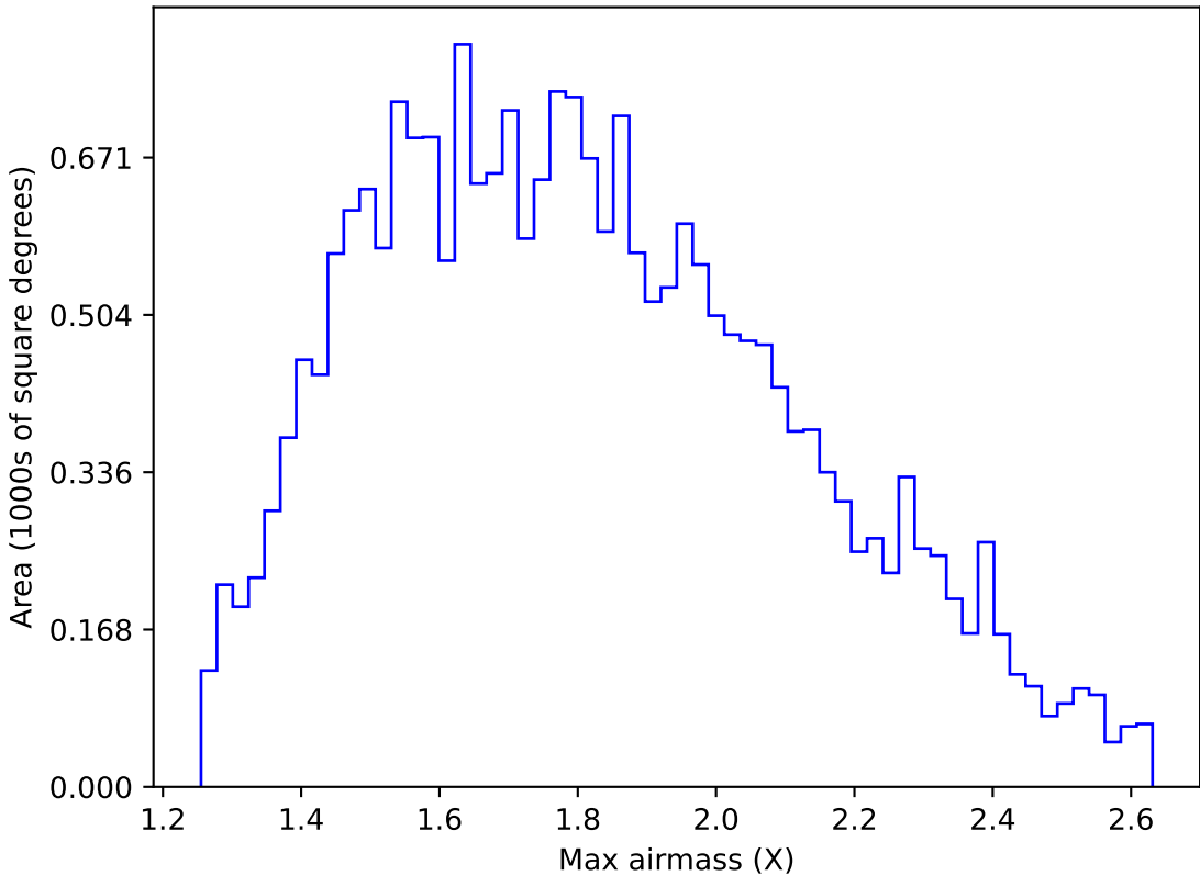
ddf_acor_sf15_lsf30_lsr20_v3.4_10yrs All sky u band: Max airmass
