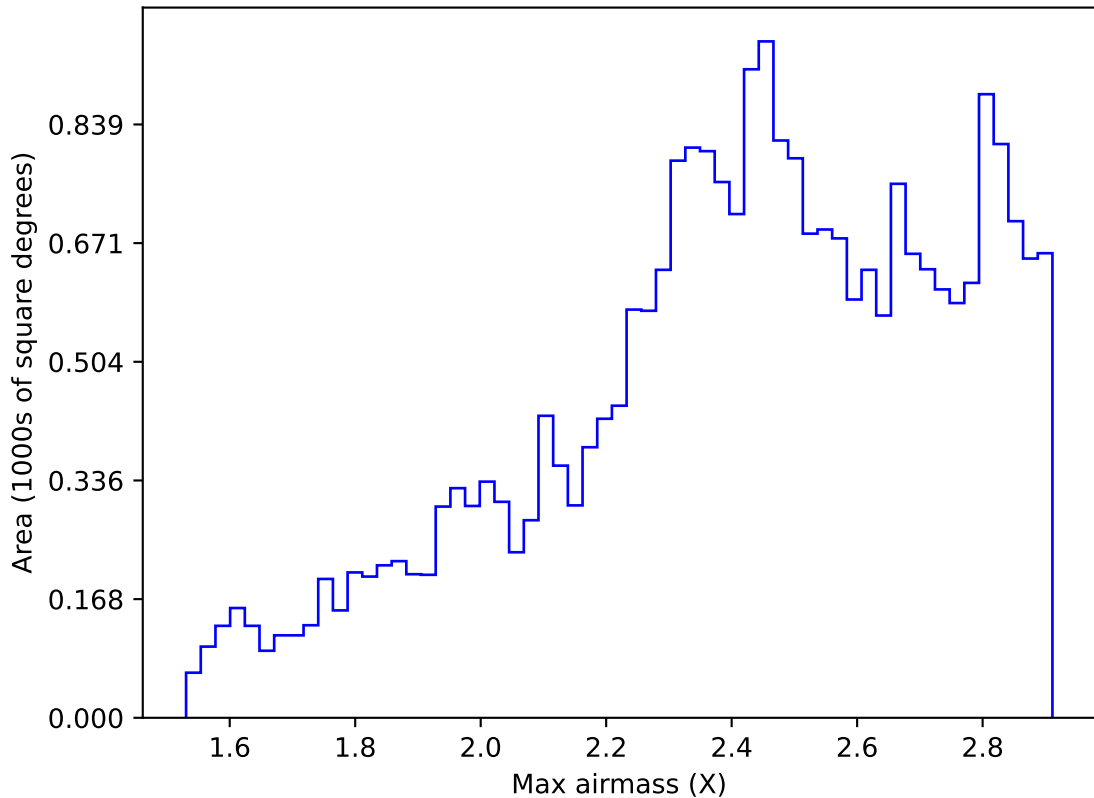
ddf_acor_sf15_lsf30_lsr20_v3.4_10yrs All sky i band: Max airmass
